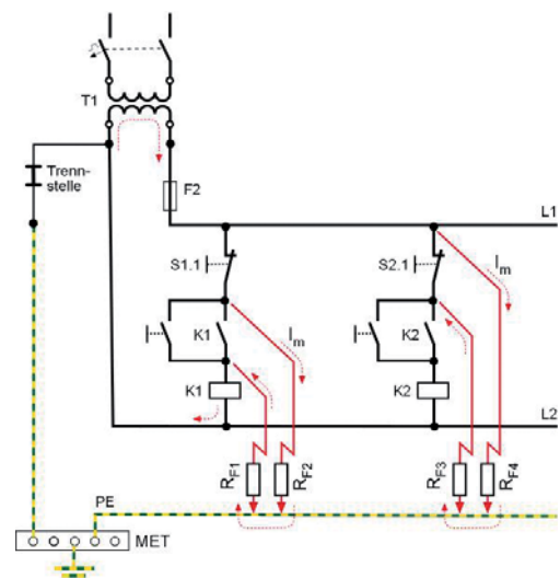
FIG. 3: Symmetrical insulation fault in an earthed control circuit (TN system)
